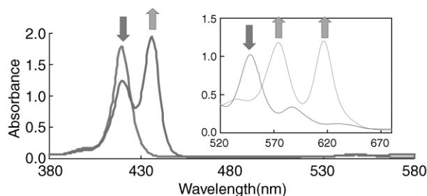
Fig. 2 UV-visible spectra of 3a (solid line, [\mathbf{3a}] = 3 \times 10^{-6} \text{ M} ) in \text{CH}_2\text{Cl}_2 , after solid/liquid extraction of NaCN; the dashed line corresponds to free 3a ( [\mathbf{3a}] = 1.5 \times 10^{-4} \text{ M} in the inset).
