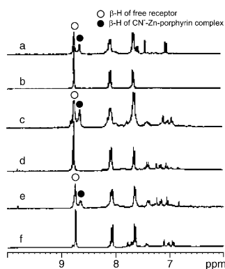
Fig. 1 Partial ^1\text{H} NMR spectra in \text{DMSO}-d_6 , checked after solid/liquid extraction of NaCN by the receptors: (a) co-receptor (ZnTPP + 3 equiv. 15BC5) + NaCN, (b) ZnTPP + NaCN, (c) 3a + NaCN, (d) 3a only, (e) 3b + NaCN, (f) 3b only.
