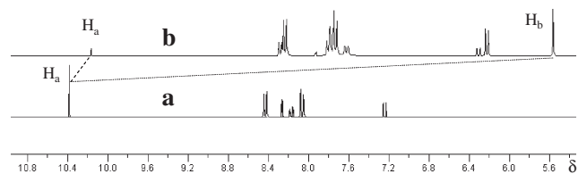
Figure 1. 1 H NMR spectral change of 1 upon addition of cyanide anion. (a) 1 only and (b) [CN^-]/[1] = 1.5 , where [1] = 5.0 mM in DMSO- d 6 at 25 °C.
