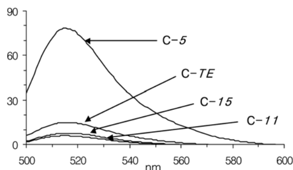
Figure 3. Fluorescence emission responses of C-5 , C-11 , C-15 and C-TE . [probe] = 1 μM, \lambda_{ex} = 490 nm.
