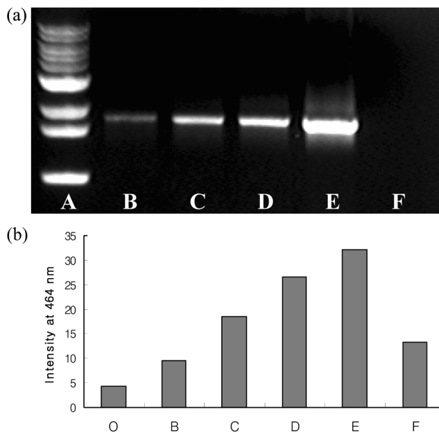
Figure 2. (a) Gel electrophoresis of finished PCR mixtures. (b) Fluorescence intensity of 1 -2Zn sensor (5 \mu M) at 464 nm upon addition of the finished PCR product mixture in 10 mM HEPES buffer (pH 7.4) at 25 ^{\circ} C: (A) Standard bp ladder, (O) 0 \mu L (B) 1 \mu L, (C) 3 \mu L, (D) 5 \mu L, (E) 9 \mu L finished PCR product mixture performed with template DNA and (F) 9 \mu L finished PCR product mixture performed without template DNA.
