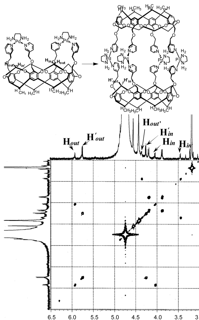
Figure 2. Partial HH COSY spectra (500 MHz, D 2 O/MeOD- d 3 , 1:5, v/v) of Pd-intra ( H out , H in , H out' , and H in' ) and Pd-inter ( H out' and H in' ) mixtures.
